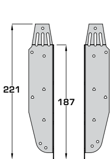
UH-195 (To suit 195 - 202mm deep open web joists)
