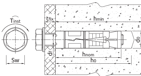
Installation in solid substrate
